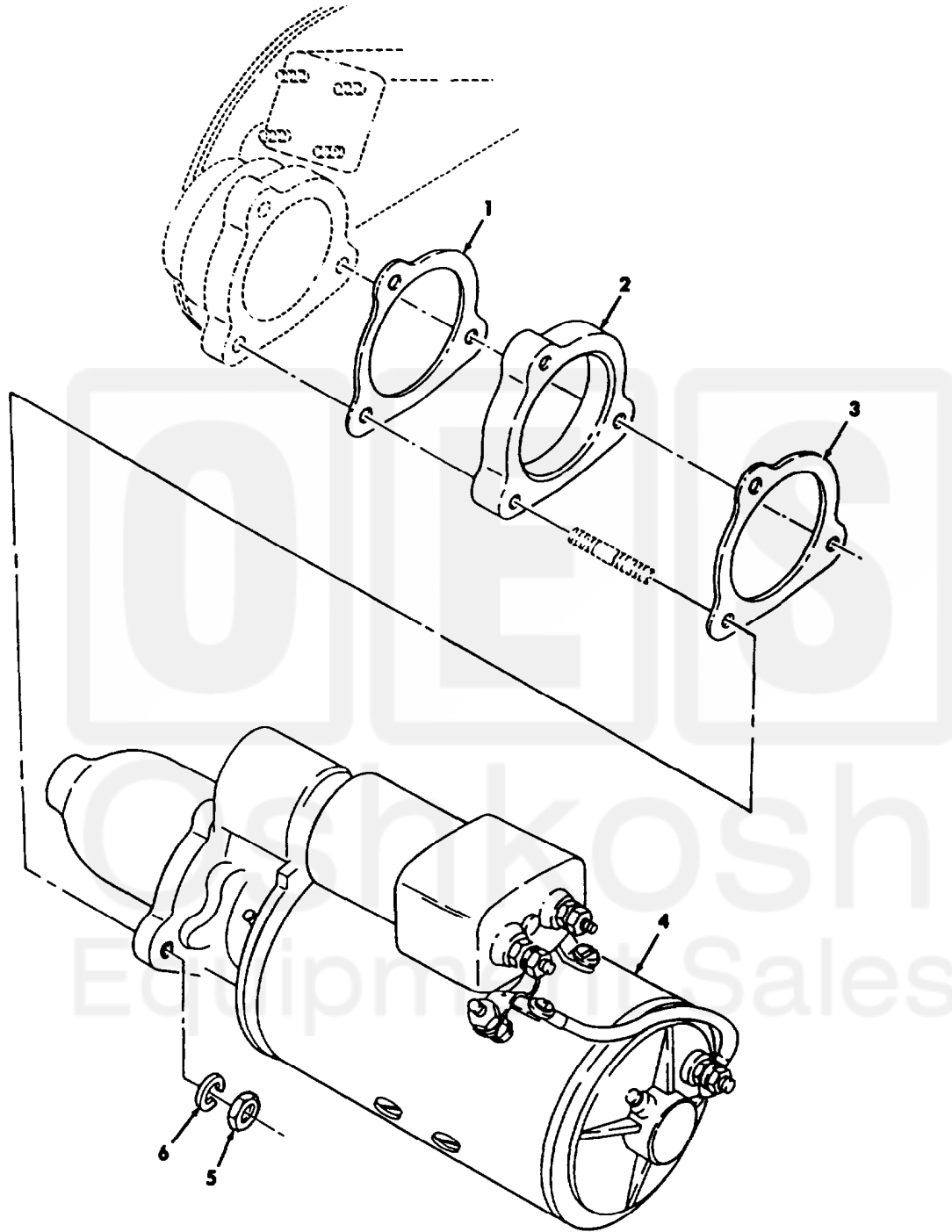
Figure 32. Starting Motor and Related Parts.
